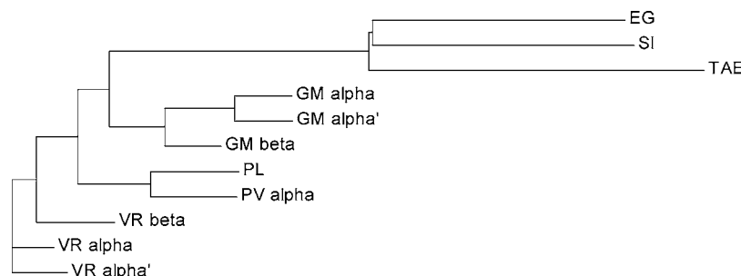
Figure 3. Phylogenetic analysis of the DNA sequences of the mungbean 8S isoforms and vicilin type cDNA from other crops using the Vector NTI software (11). Legends: Vigna radiata (VR) 8S \alpha , \alpha' , and \beta , sequences from this paper; P. vulgaris (PV \alpha ) \alpha type (X02980), ref 19; P. lunatus (PL \alpha ) \alpha type (U01122), ref 29; G. max (GM \alpha ) \alpha , \beta -conglycinin (AB008678); G. max (GM \alpha' ) \alpha' , \beta -conglycinin (AB008680); G. max (GM \beta ) \beta , \beta -conglycinin (AB008679) (22); T. aestivum (TAE) (AAA34269.1), ref 30; Sesame indicum (SI) (AAK15089) (31); Elaeis guineensis (EG) (AAK28402.1) (32).
